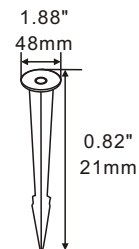
AB-007 Die-cast stake
