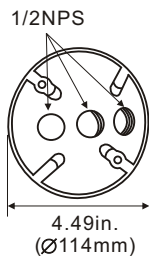
OB-003 Junction Box
